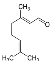
Citral
