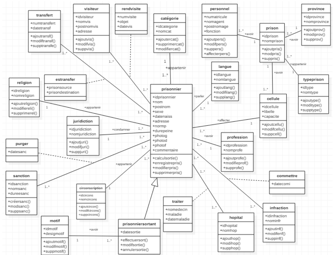
FIGURE 3.7 – Diagramme des classes
